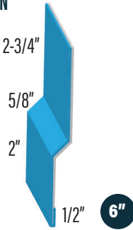
WALL TRANSITION WEATHERSHIELD WSWT
