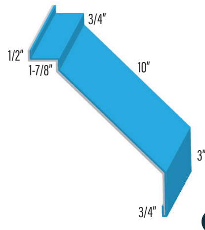
CANNONBALL TRACK COVER FACE DOUBLE TRACK
