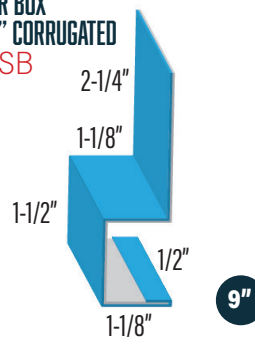
STARTER BOX WF-HF/PROLOK HFSB
