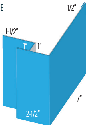
CANNONBALL TRACK COVER FACE KWIK-FRAME SINGLE TRACK
