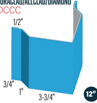
CORNER POST 1 CP1
