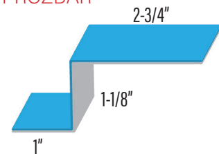
Z BAR TRIM SUPPORT (226A) PROLOK PROZBAR
