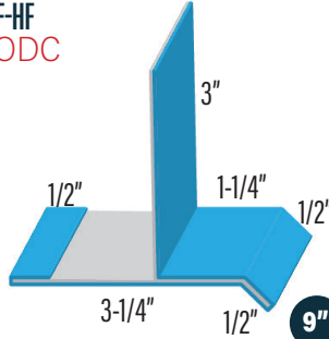
SKIRT MESA WM2RIB
