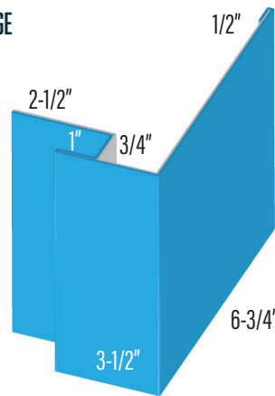
CANNONBALL TRACK COVER FACE DOUBLE TRACK
