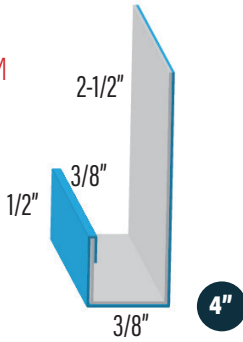
J TRIM 1 - COLOR 1 SIDE WF-7/8" CORRUGATED CORJT1
