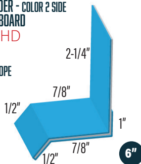
HEADER - COLOR 2 SIDE WF-12-36 1236HD
