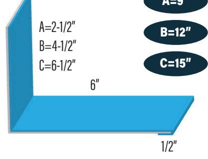
SKYLITE 2-A, B, C WF-7/8" CORRUGATED CORSKY2-A,B,C
