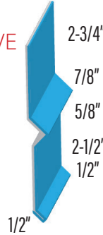
BASE TO CONCRETE BTC
