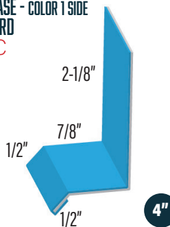
WALL BASE - COLOR 1 SIDE WF-12-36 1236DC
