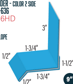
REVERSE WALL BASE AND HEADER EX. (Profile)DCR or (Profile)HDR
