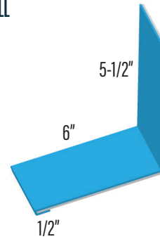
SIDE WALL WF-7/8" CORRUGATED CORSW
