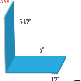
CHIMNEY SIDEWALL WF-636 636CHSW
