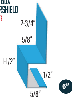
STARTER BOX WF-12-36 1236SB
