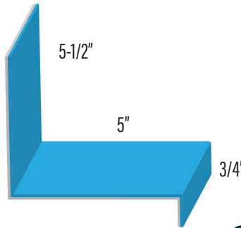
CHIMNEY SIDEWALL DURACLAD/ALLCLAD/DIAMOND DCCHSW
