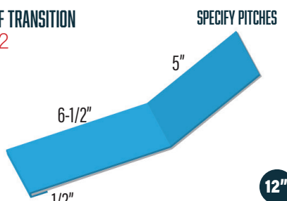
ROOF TRANSITION RT2L
