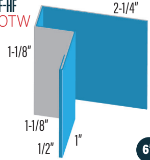
Z BAR TRIM SUPPORT (226A) PROLOK PROZBAR
