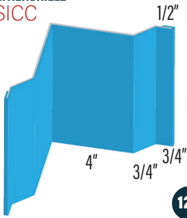
INSIDE CORNER POST 1 ICP1
