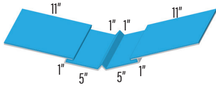
W VALLEY 36" HOOK WVH36
