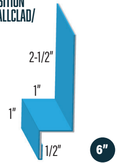
WALL TRANSITION WF-636 636WT
