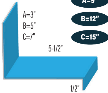
SKYLITE 2-A, B, C WEATHERSHIELD WSSKY2-A,B,C
