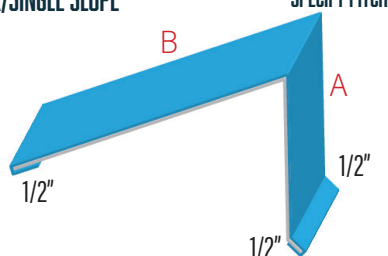
ROOF TRANSITION RT1
