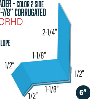
REVERSE WALL BASE AND HEADER EX. (Profile)DCR or (Profile)HDR
