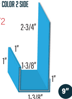
J TRIM 2 - COLOR 2 SIDE WF-636 636JT2
