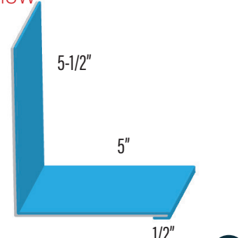
CHIMNEY SIDEWALL WF-7/8" CORRUGATED CORCHSW
