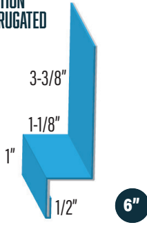
WALL TRANSITION WF-HF/PROLOK HFWT
