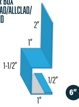
STARTER BOX WF-636 636SB
