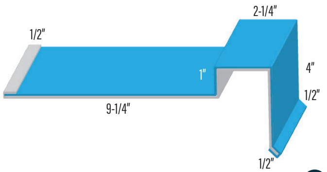
WF-7/8" CORRUGATED CORPROW
