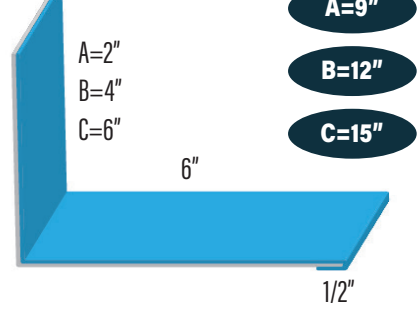
SKYLITE 2-A, B, C WF-636 636SKY2-A,B,C
