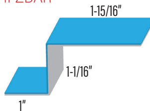
PANEL SUPPORT WF-HF HFZBAR
