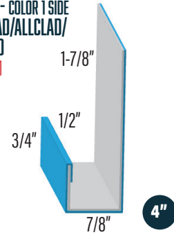
J TRIM 1 - COLOR 1 SIDE WF-636 636JT1
