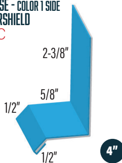
WALL BASE - COLOR 1 SIDE WF-HF/PROLOK HFDC
