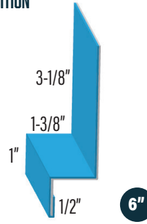
STARTER BOX WF-7/8" CORRUGATED CORSB
