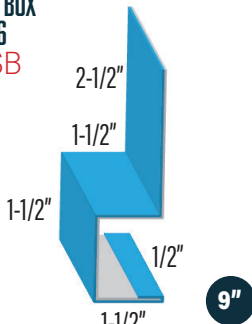
STARTER BOX WF-636 636SB
