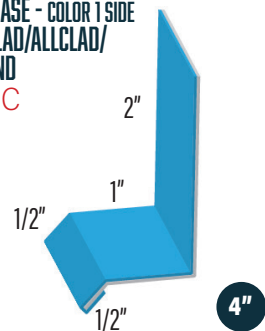
WALL BASE - COLOR 1 SIDE WF-636 636DC
