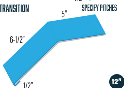
ROOF TRANSITION RT2
