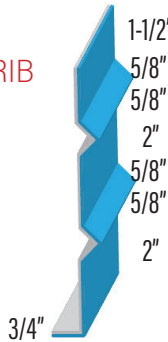
PANEL SUPPORT PROBOARD PBZBAR
