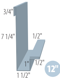
DROP FASCIA PBDF
