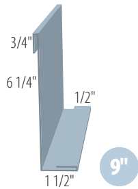
FLUSH FASCIA PBFF
