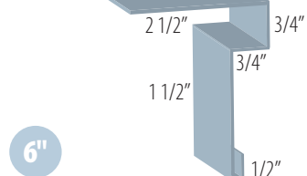
WALL TO SOFFIT PBWTS
