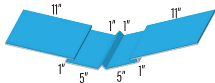
W VALLEY 36" HOOK WVH36
