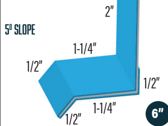
HEADER - COLOR 2 SIDE WF-HF/PROLOK HFHD
