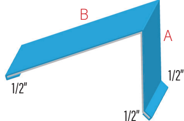
ROOF TRANSITION RT1
