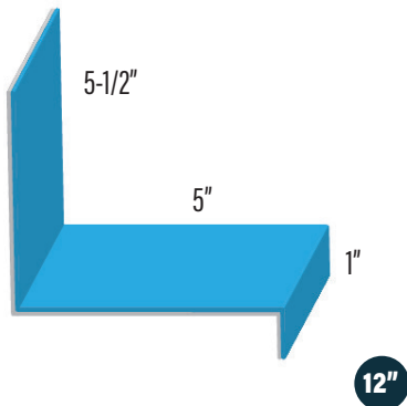
CHIMNEY SIDEWALL PROLOK PRCHSW
