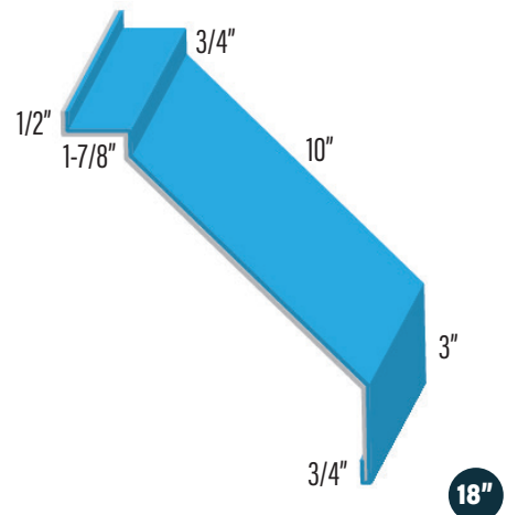
CANNONBALL TRACK COVER DOUBLE
