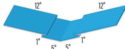
V VALLEY 36" HOOK VH36
