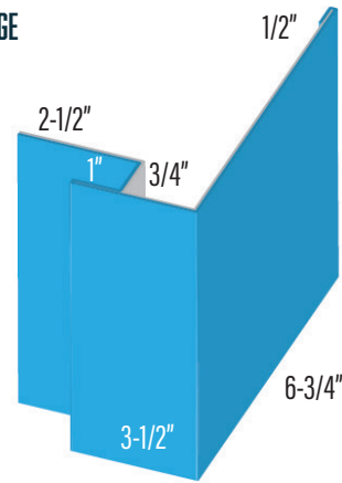
CANNONBALL TRACK COVER DOUBLE
