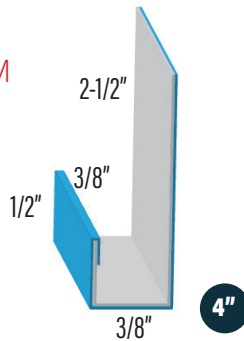
J TRIM 1 - COLOR 1 SIDE WF-7/8" CORRUGATED CORJT1
