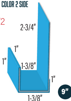
J TRIM 2 - COLOR 2 SIDE WF-636 636JT2
