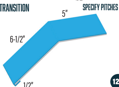
ROOF TRANSITION RT2
