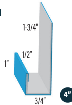
J TRIM 1 - COLOR 1 SIDE WF-12-36 1236JT1
