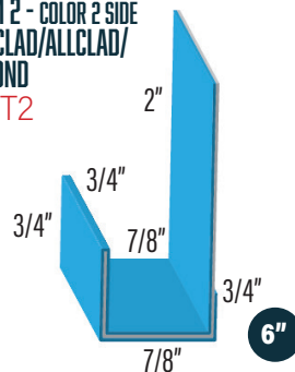
J TRIM 2 - COLOR 2 SIDE WF-636 636JT2
