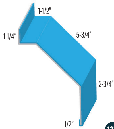
CANNONBALL TRACK COVER BIGG
