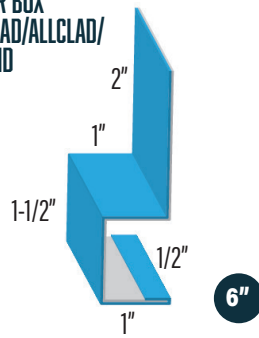
STARTER BOX WF-636 636SB
