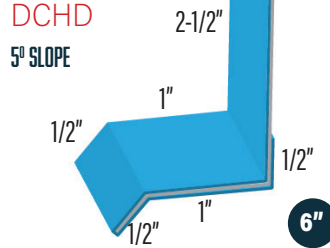
HEADER - COLOR 2 SIDE WF-636 636HD
