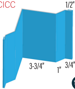
INSIDE CORNER POST 2 ICP2
