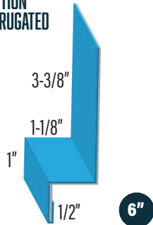
WALL TRANSITION WF-HF/PROLOK HFWT
