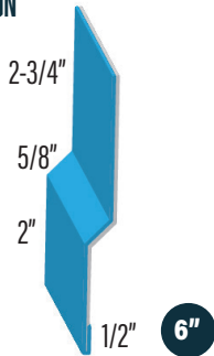
WALL TRANSITION WEATHERSHIELD WSWT
