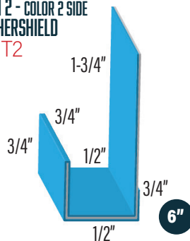
J TRIM 2 - COLOR 2 SIDE WF-12-36 1236JT2
