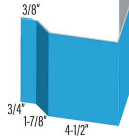
CORNER POST 2 CP2
