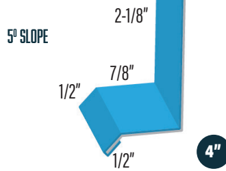
WALL BASE - COLOR 1 SIDE WF-12-36 1236DC
