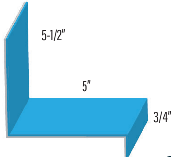
CHIMNEY SIDEWALL DURA-CLAD/ALL-CLAD/DIAMOND DCCHSW
