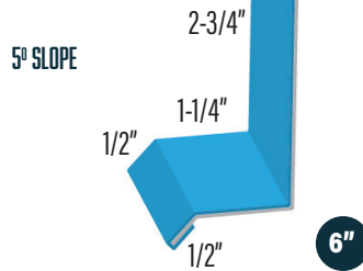
HEADER - COLOR 2 SIDE PROBOARD PBHD
