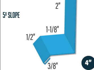
HEADER - COLOR 2 SIDE WEATHERSHIELD WSHD
