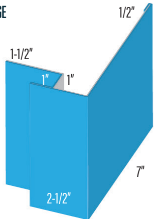
CANNONBALL TRACK COVER FACE
