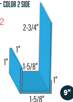
J TRIM VENTED JTV
