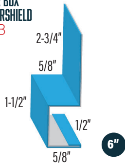
STARTER BOX WF-12-36 1236SB
