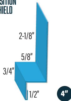
WALL TRANSITION WF-HF/PROLOK HFWT
