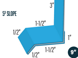
HEADER - COLOR 2 SIDE WF-12-36 1236HD
