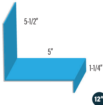
CHIMNEY SIDEWALL WF-12-36 1236CHSW
