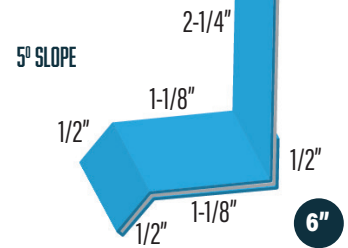
REVERSE WALL BASE AND HEADER EX. (Profile)DCR or (Profile)HDR
