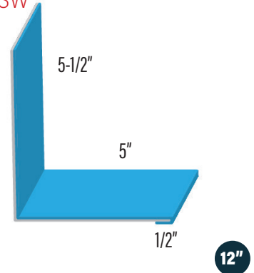
CHIMNEY END WALL CHEW
