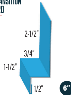
WALL TRANSITION WF-12-36 1236WT
