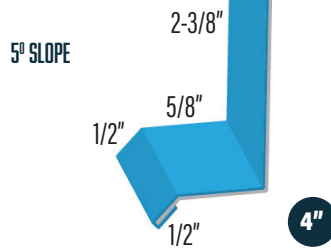
WALL BASE - COLOR 1 SIDE WF-HF/PROLOK HFDC
