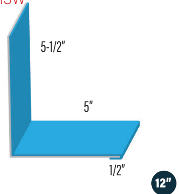
CHIMNEY SIDEWALL WF-636 636CHSW
