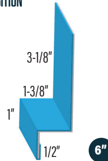
STARTER BOX WF-7/8" CORRUGATED CORSB
