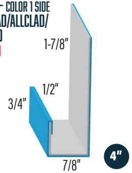
J TRIM 1 - COLOR 1 SIDE WF-636 636JT1
