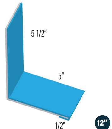
CHIMNEY END WALL CHEW
