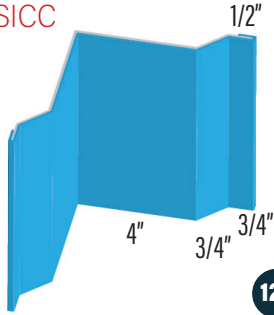
INSIDE CORNER POST 1 ICP1
