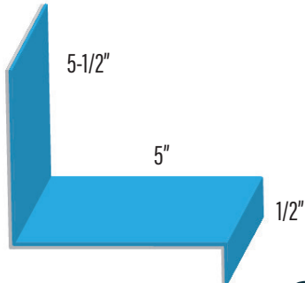
CHIMNEY SIDEWALL WEATHERSHIELD WSCHSW
