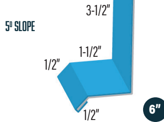
HEADER - COLOR 2 SIDE DURACLAD/ALLCLAD/ DIAMOND DCHD
