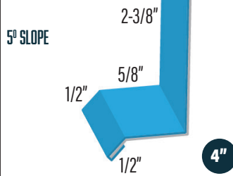
WALL BASE - COLOR 1 SIDE WF-7/8" CORRUGATED CORDC
