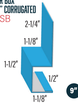
STARTER BOX WF-HF/PROLOK HFSB
