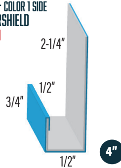
J TRIM 1 - COLOR 1 SIDE WF-HF HFJT1
