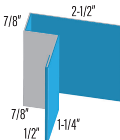
INSIDE CORNER TRIM 1 ICT1
