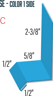
WALL BASE - COLOR 1 SIDE WF-7/8" CORRUGATED CORDC
