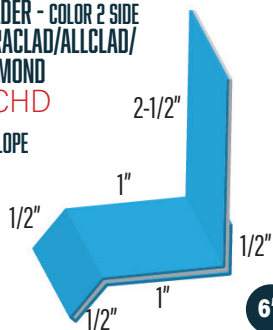
HEADER - COLOR 2 SIDE WF-636 636HD
