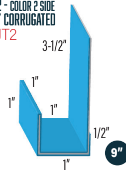
J TRIM VENTED JTV
