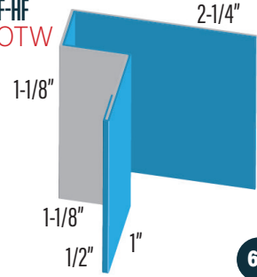
Z BAR TRIM SUPPORT (22GA) PROLOK PROZBAR
