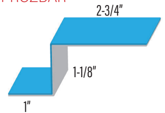
Z BAR TRIM SUPPORT (22GA) PROLOK PROZBAR
