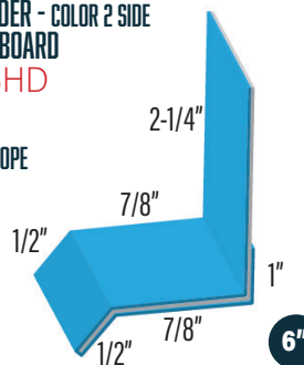
HEADER - COLOR 2 SIDE WF-12-36 1236HD
