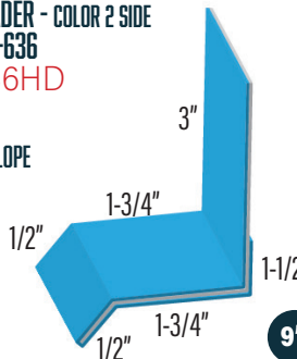
REVERSE WALL BASE AND HEADER EX. (Profile)DCR or (Profile)HDR
