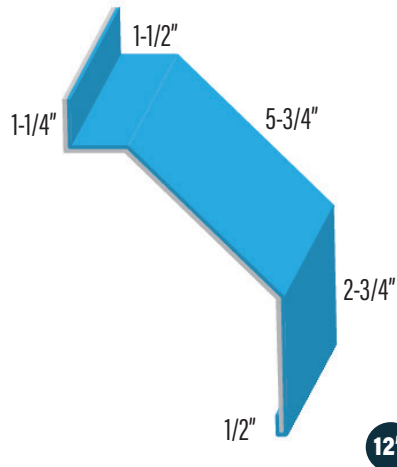
CANNONBALL TRACK COVER BIGG
