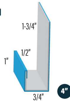
J TRIM 1 - COLOR 1 SIDE WF-12-36 1236JT1
