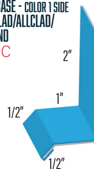
WALL BASE - COLOR 1 SIDE WF-636 636DC
