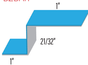
PANEL SUPPORT PROBOARD PBZBAR
