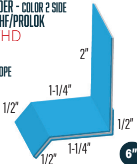
HEADER - COLOR 2 SIDE WF-12-36 1236HD
