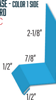
WALL BASE - COLOR 1 SIDE WF-12-36 1236DC
