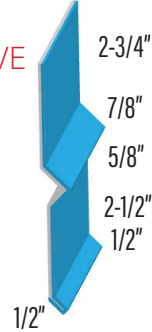
BASE TO CONCRETE BTC
