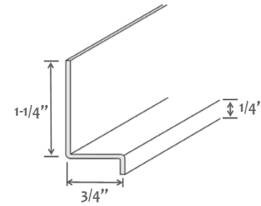
Base Trim
