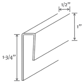
J-Trim
