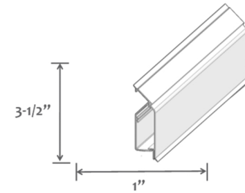
Multi-function Trim
