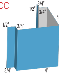
J TRIM VENTED JTV.75
