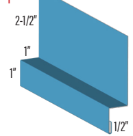
WALL TRANSITION DCWT
