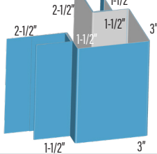
CORNER POST DCIP
