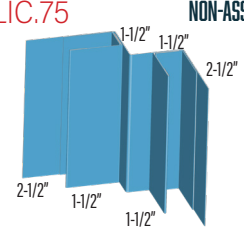
CORNER POST DCOP
