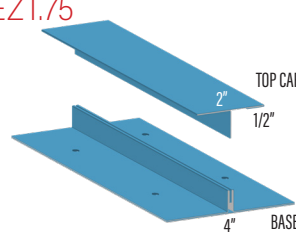
J TRIM VENTED JTV.75
