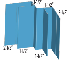
I/S CORNER QLIC1
