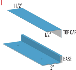
I/S CORNER QLIC1
